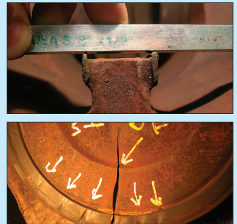
Cryogenic testing.
